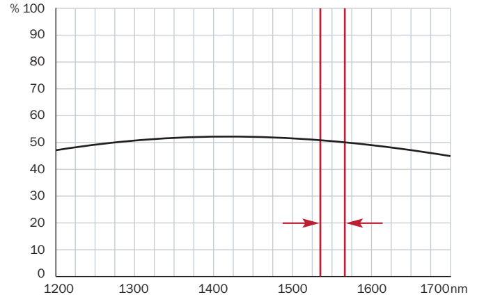
Wavelength dependence of Coupling Ratio of symmetrical C-Band Coupler
